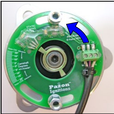
Rotate trigger assembly fully counter-clockwise
