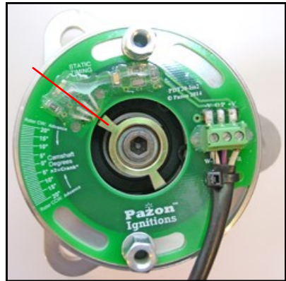
Rear piston @ TDC on compression stroke, Align centre of rotor tab with static timing lead, tighten rotor cap head screw
