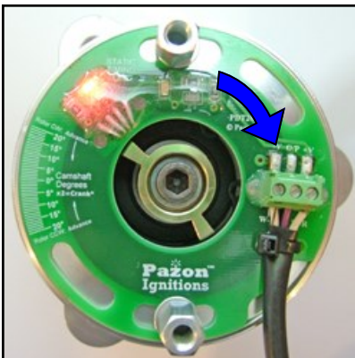
Rotate trigger very slowly CLOCKWISE until red static timing led turns ON STOP ROTATING TIGHTEN PILLAR FIXINGS
